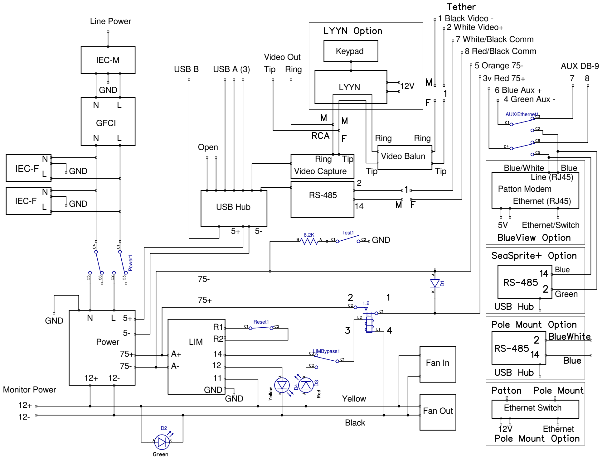
Fully Optioned Pro 4 Control Panel
